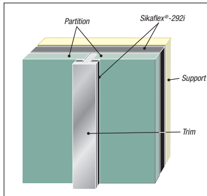
Fig. 1 Sikaflex®-292i bead application for bonding to the support
