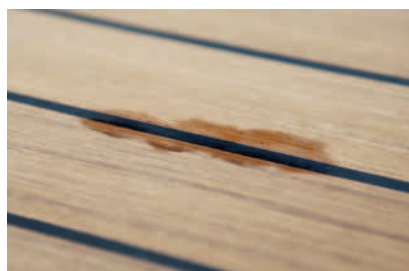
Fig. 32 Discolouration of the wood is a tell-tale sign of a failed or damaged joint in this teak deck
