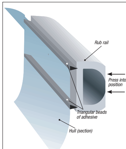
Fig. 1 Assembly of a rub rail
