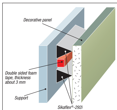
Fig. 1 Bonding a decorative panel vertically
