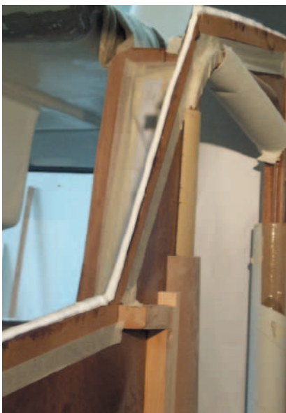
Fig. 3 Sikaflex®-292i applied to a lightweight panel prior to fitting
