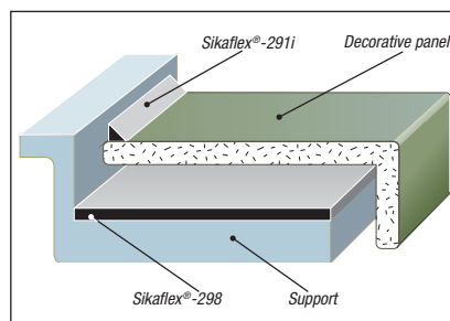
Fig. 2 Bonding a decorative panel horizontally
