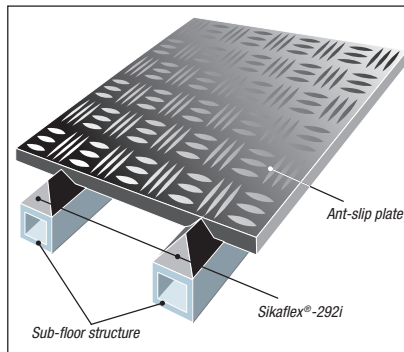
Fig. 2 Bonding anti-slip plates to the sub-floor structure
