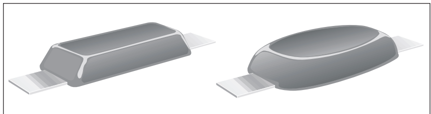
Fig. 3 Examples of weld-on sacrificial anodes
