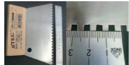
Fig. 11 Hand application picture comb trowel and comb trowel detail
