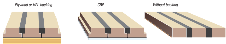
Fig. 21 Typical prefabricated teak deck profiles
