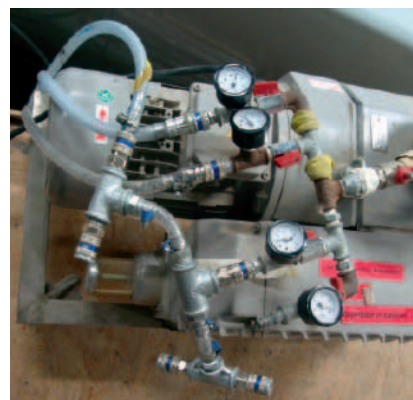
Fig. 16 Vacuum equipment
