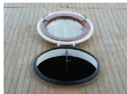
Fig. 3 A port-hatch, both bonded and sealed using Sikaflex®
